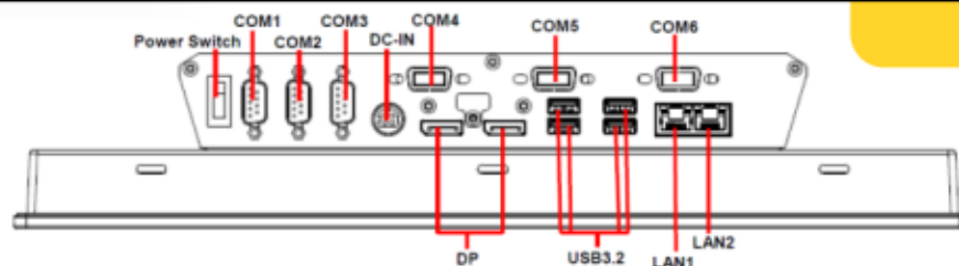
I/O Panel
